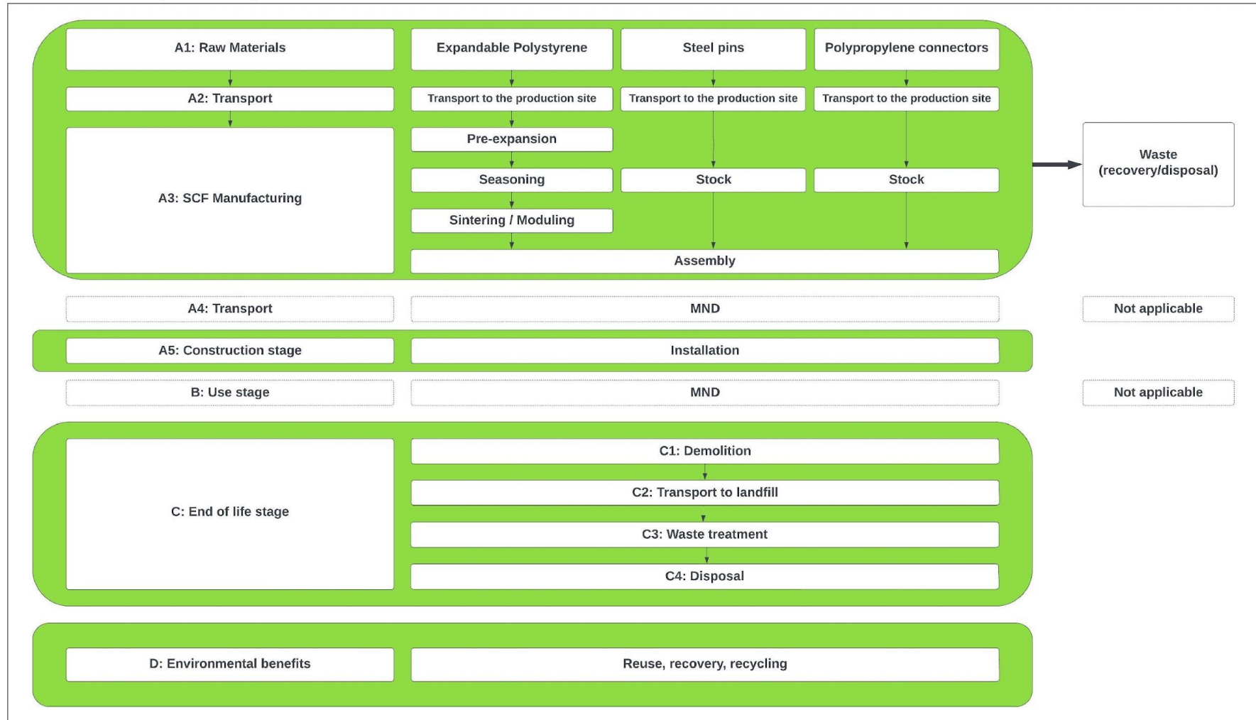
Flow chart of production system
